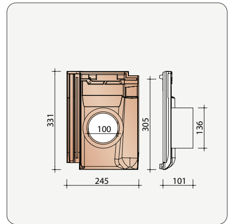
BCFL8740 Kokerpan Ø 100 mm
