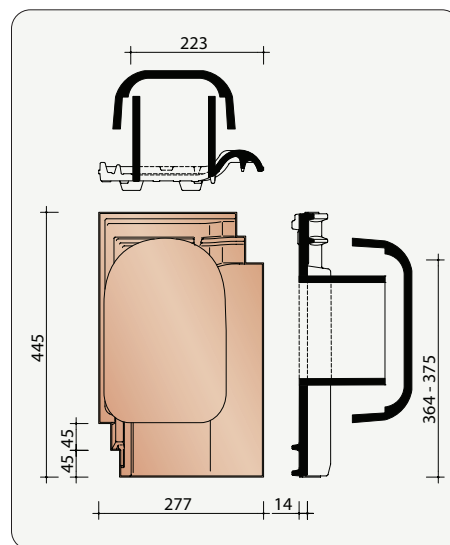
HHAR8728 Kit kokerpan Ø 125 mm + kapje + onderdakadapter
