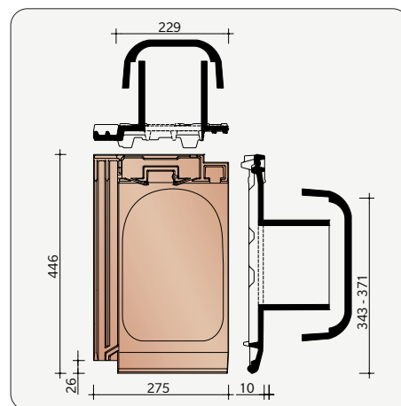
HMIK8728 Kit kokerpan Ø 125 mm + kapje + onderdakadapter
